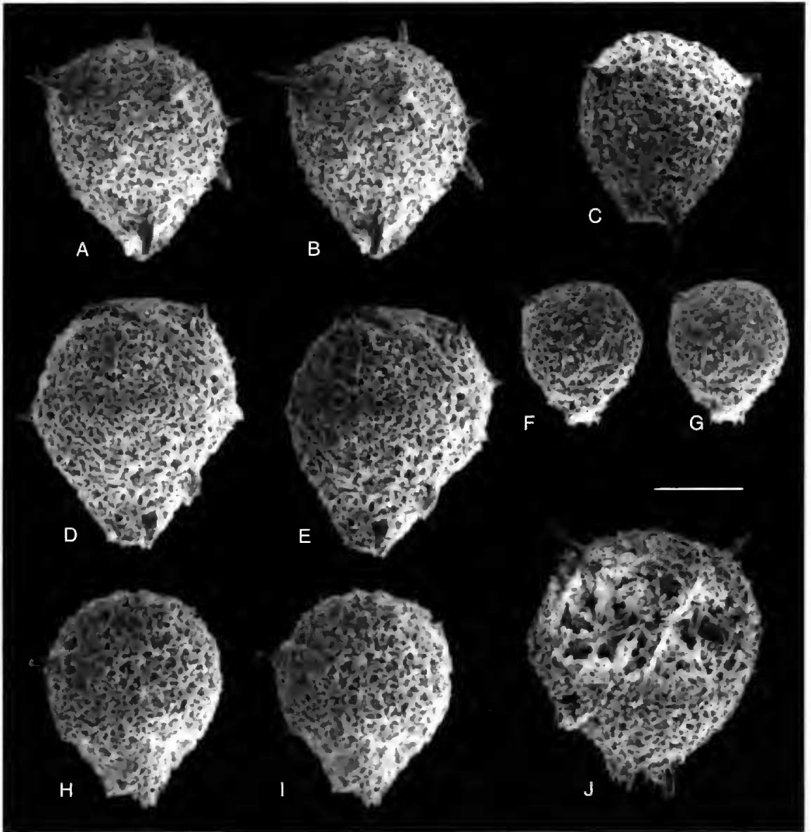
FIG. 13. — Glomeropyle mahinepuaensis Aita, n. sp. ; A, B, holotype, stereograph (photo Nos 31111, 31112); C, photo No. 31119; D, E, paratype, stereograph (photo Nos 31113, 31114); F, G, paratype, stereograph (photo Nos 31129, 31130); H, I, paratype, stereograph (photo Nos 31116, 31115); J, photo No. 31117. Sample MAH-3.5, Unit 2, Mahinepua Peninsula, North Island, New Zealand. Scale bar: 100 \mu m.
